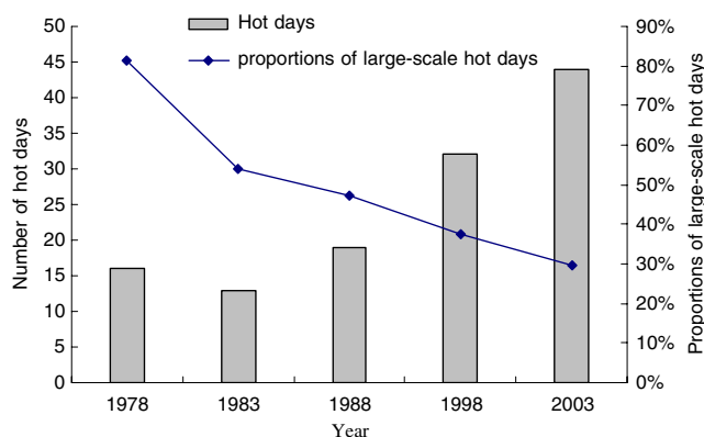
Fig. 5 The number of hot days ( >35^{\circ}\text{C} ) and the proportion of large-scale hot days ( >35^{\circ}\text{C} at eight or more stations) during the five hottest years on record
