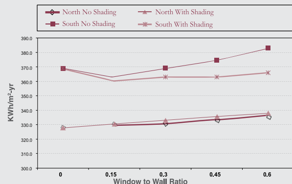
Fig. 6: Impact of Orientation and Shading on Annual Electricity Consumption
