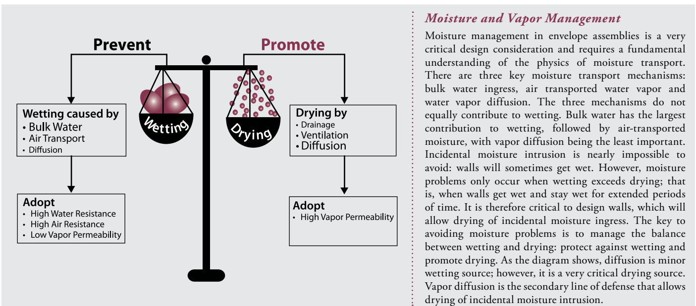
Fig. 4: Moisture and Vapor Management Source: DuPont
