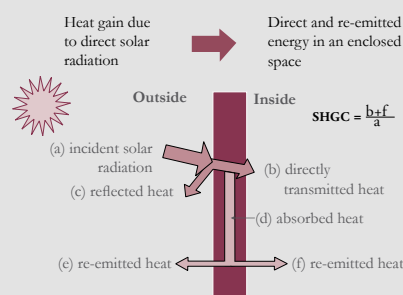
Fig. 2: Solar Heat Gain Coefficient
